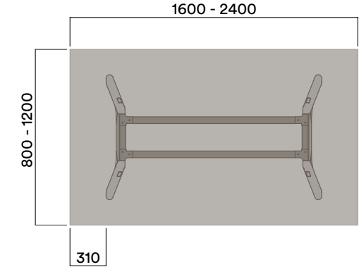
TQT-1050 4 Leg
