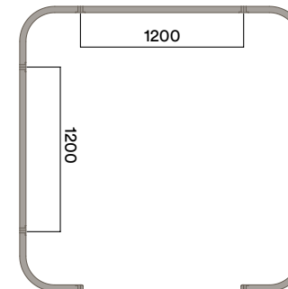
TQB-2424 C-Shape 2400×2400
