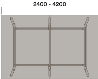
TQT-1051-XXL 6 Leg
