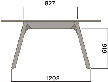
TQT-1053-XL 10 Leg
