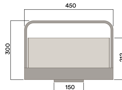
TQA-5700 Terrarium
