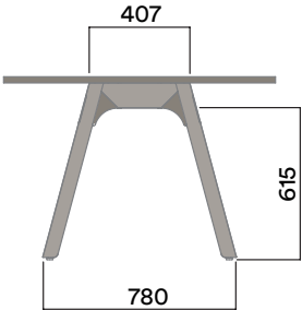
TQT-1053 10 Leg
