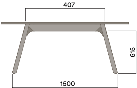
TQT-1053-XXL 10 Leg
