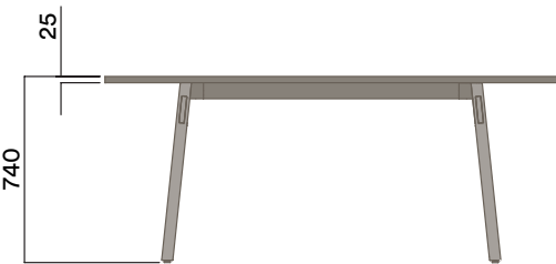
TQT-1051-XL 6 Leg
