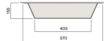
Cut-out in Worktop
