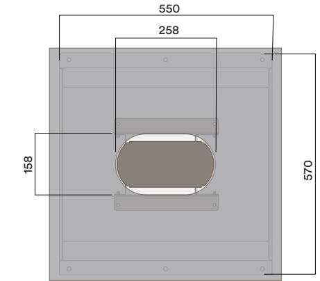
Cut-out in Worktop
