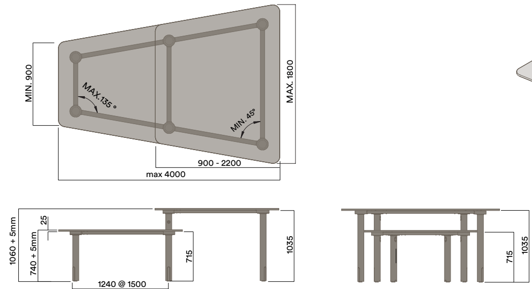
RLA-1051-MZ 6 Leg - Mezzanine Table
