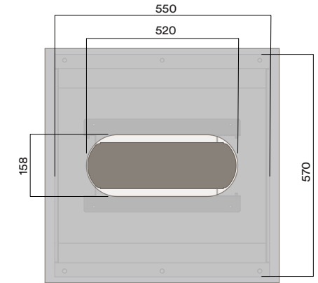
Cut-out in Worktop
