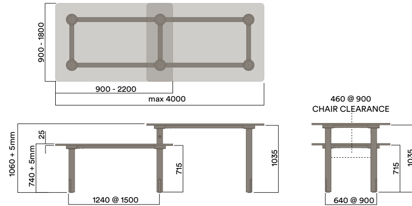
RLD-1051-MZ 6 Leg - Mezzanine Table
