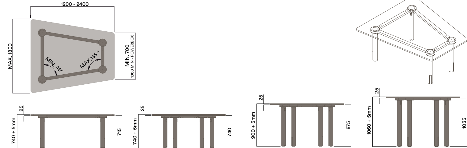
RLA-1050 Adjustable Hub Frame
