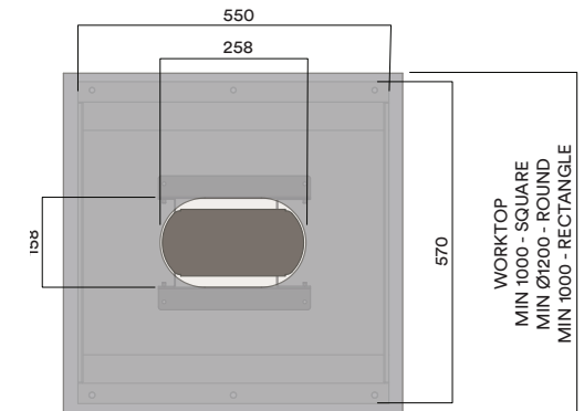
Cut-out in Worktop
