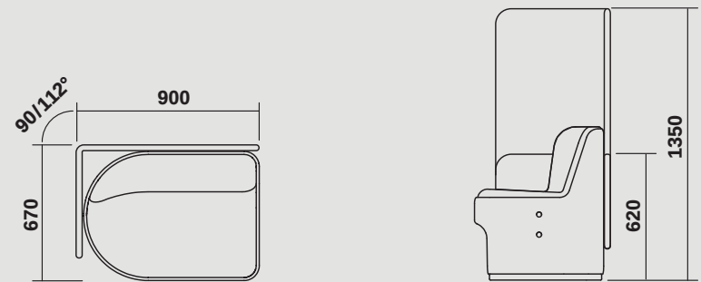
CIR-M-1020-LHS-LB/HB WITH LOW - OR - HIGH PRIVACY SCREEN
