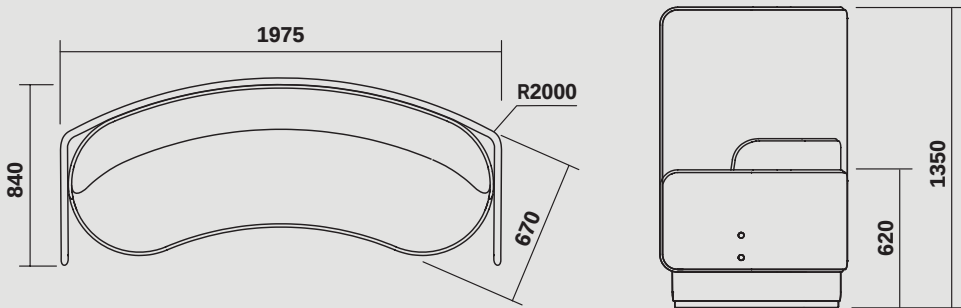
CIR-L-3020 WITH LOW - OR - HIGH PRIVACY SCREEN
