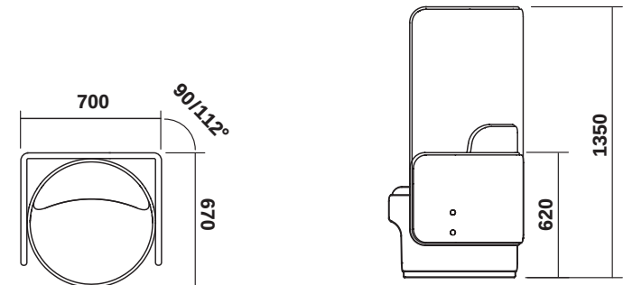
CIR-L-1010-LB/HB WITH LOW - OR - HIGH PRIVACY SCREEN
