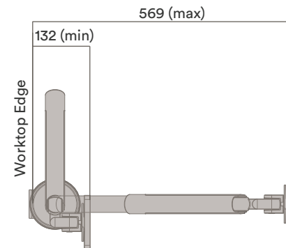
Arm Extension
