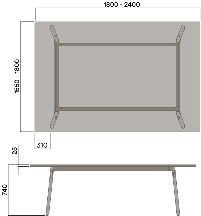
TQT-1050-XXL 4 Leg 740 (standard height)
