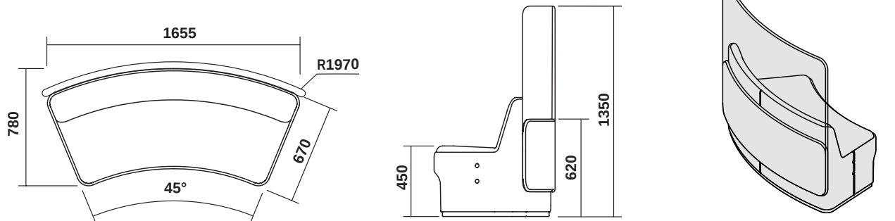
CIR-M-2050 CIRCOLO MODULAR - DOUBLE SEAT - 45DEG CONVEX CURVE
