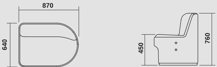
CIR-O-1020-RHS CIRCOLO MODULAR - SINGLE SEAT D-END RHS
