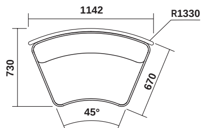
CIR-M-1040-LB/HB WITH LOW - OR - HIGH PRIVACY SCREEN
