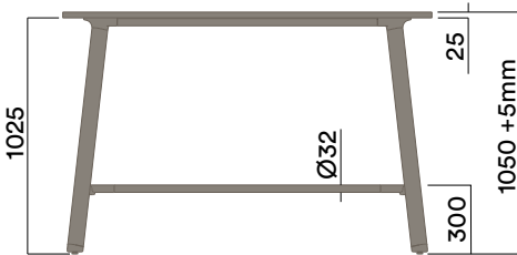
ROW-10-1100/1200/1300 1050 (standing height)
